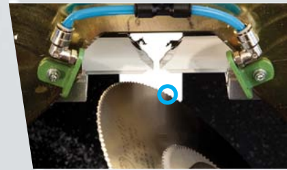
Cutting oil spray system
