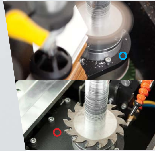
Cutting oil spray system
