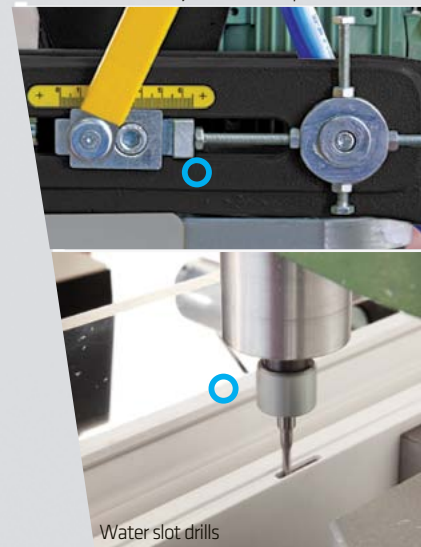
Mechanical drills adjustment stopers
