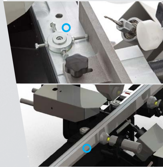
Pneumatic profile clamping system
